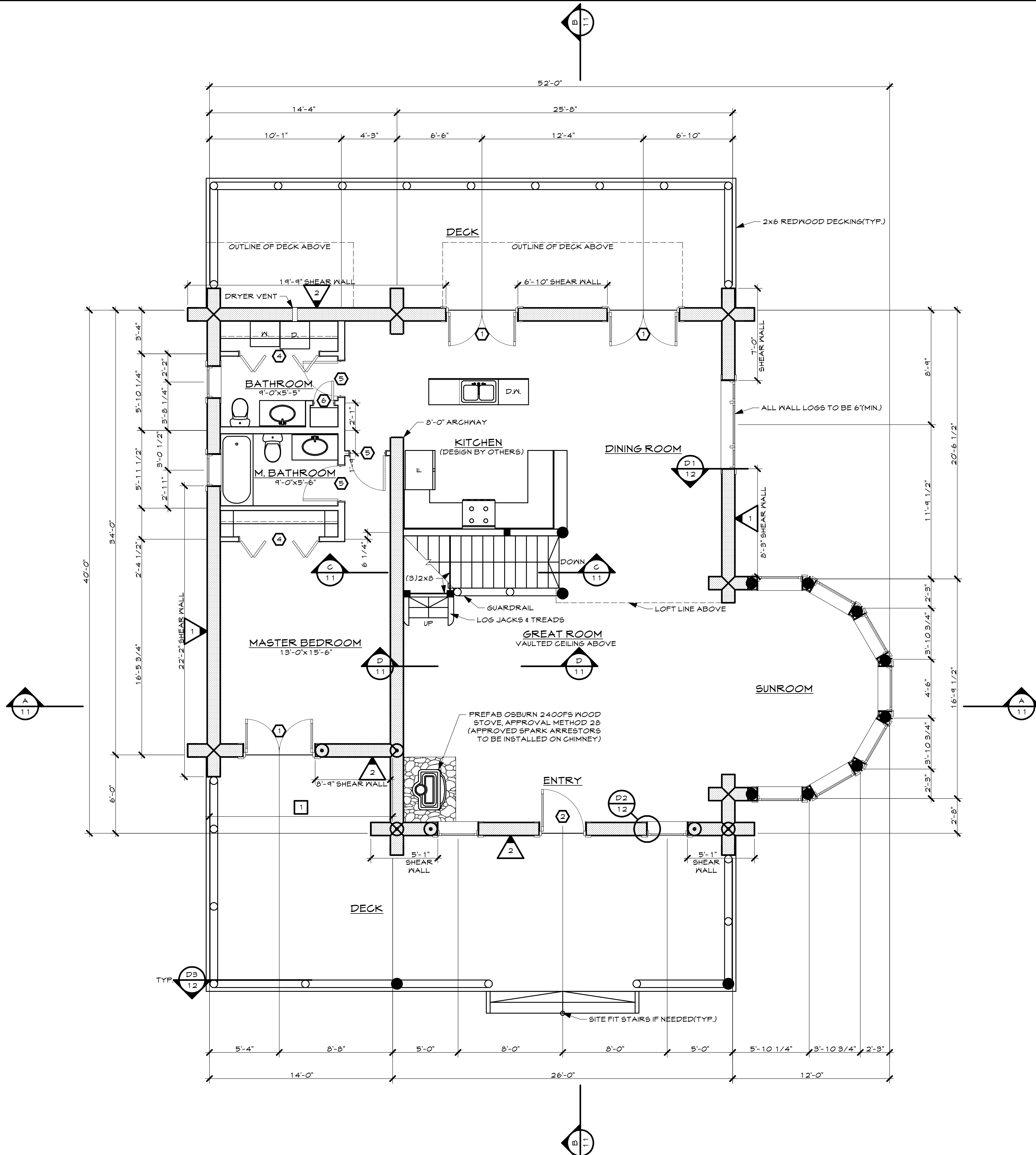
MAIN LEVEL FLOOR PLAN SCALE: 1/4" = 1'-0"
